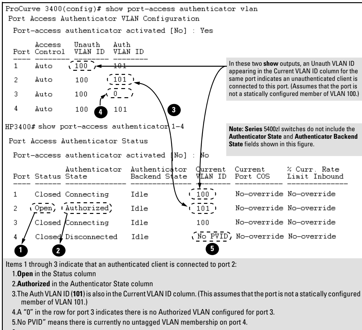
Figure 12-17. Example Showing Ports Configured for Open VLAN Mode
